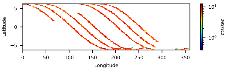
30902026004: 3 to 120 keV
