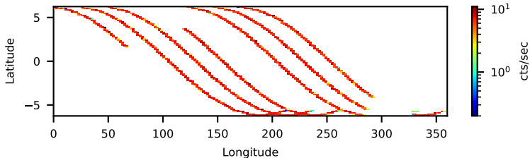
30902026004: 3 to 10 keV
