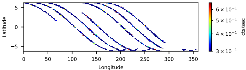
30902026004: 30 to 120 keV
