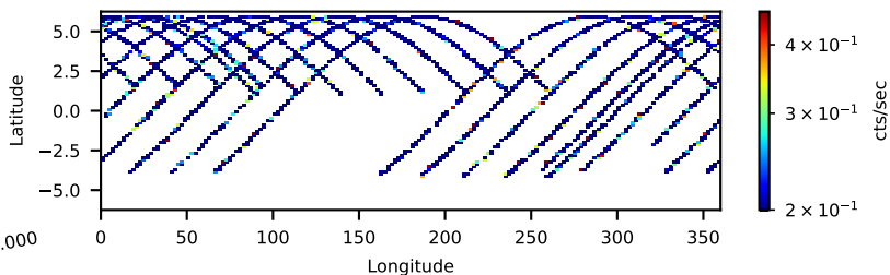
30901045002: 30 to 120 keV
