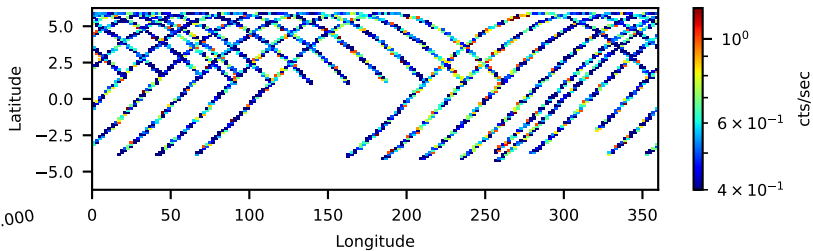
30901045002: 3 to 10 keV
