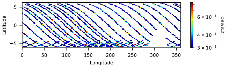
30901029002: 30 to 120 keV
