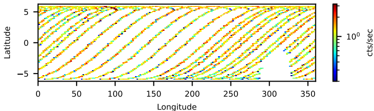
30901024002: 3 to 10 keV
