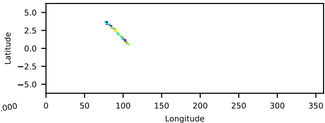
30802017005: 3 to 10 keV
