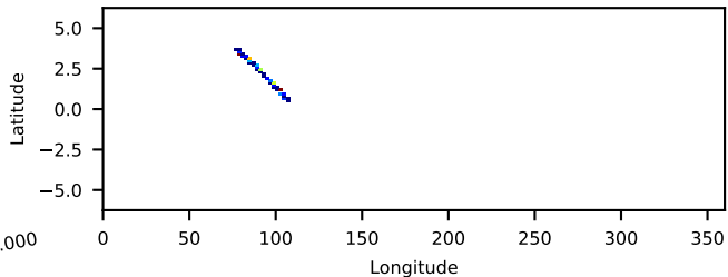
30802017005: 30 to 120 keV
