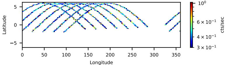
30702017006: 30 to 120 keV
