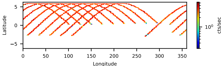
30702017002: 3 to 10 keV
