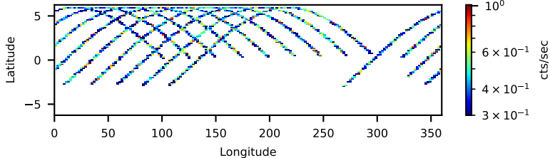
30702017002: 30 to 120 keV
