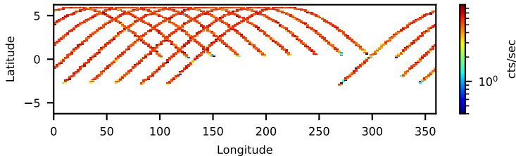
30702017002: 3 to 120 keV
