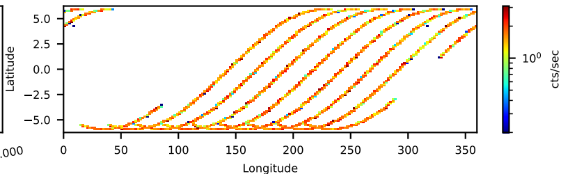
30602022004: 30 to 120 keV
