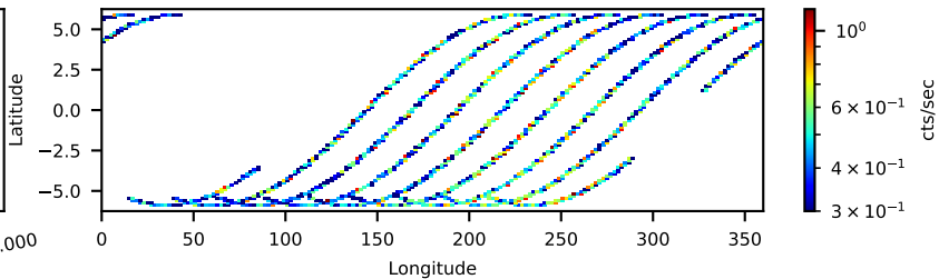
30602022004: 30 to 120 keV
