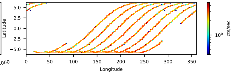
30602022004: 3 to 10 keV
