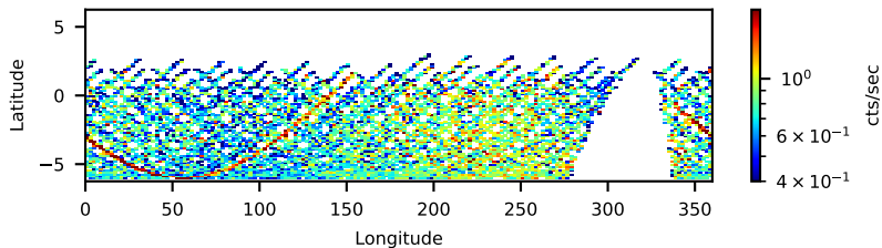
30601025002: 3 to 120 keV
