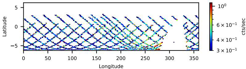
30601019002: 30 to 120 keV
