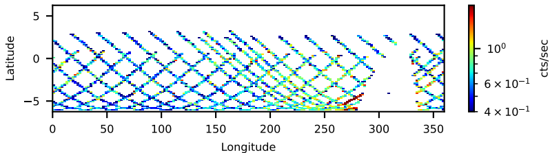
30601019002: 3 to 120 keV
