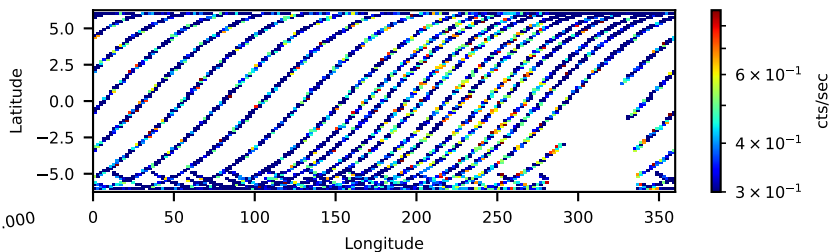
30460019002: 30 to 120 keV
