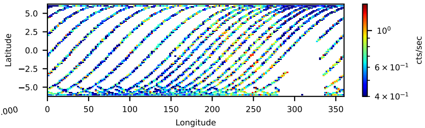
30460019002: 3 to 10 keV
