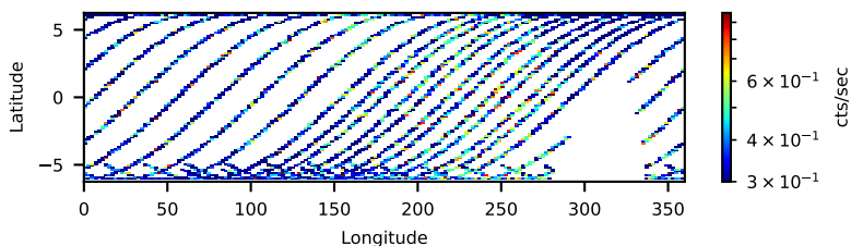
30460019002: 30 to 120 keV
