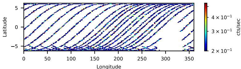
30460019002: 3 to 10 keV
