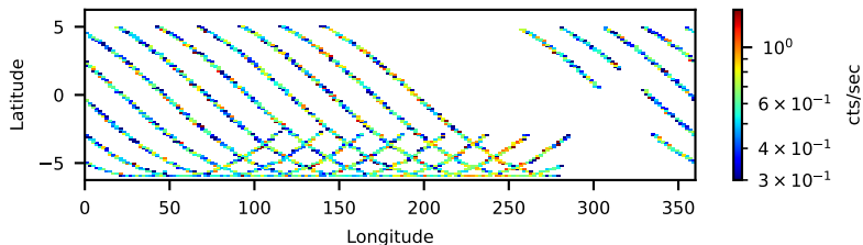
30460015002: 30 to 120 keV
