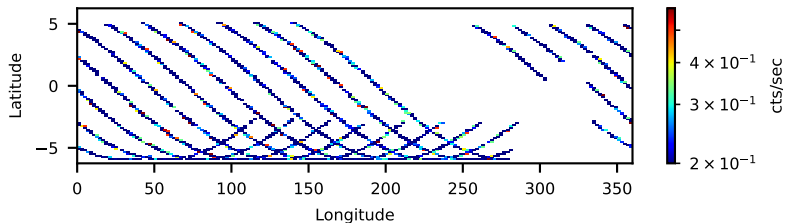
30460015002: 3 to 10 keV
