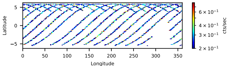
30360002002: 3 to 10 keV
