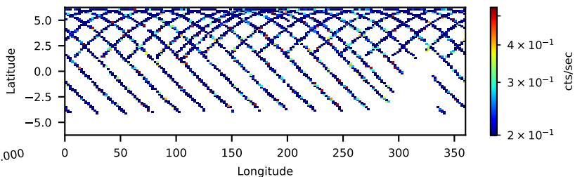
30302023004: 30 to 120 keV
