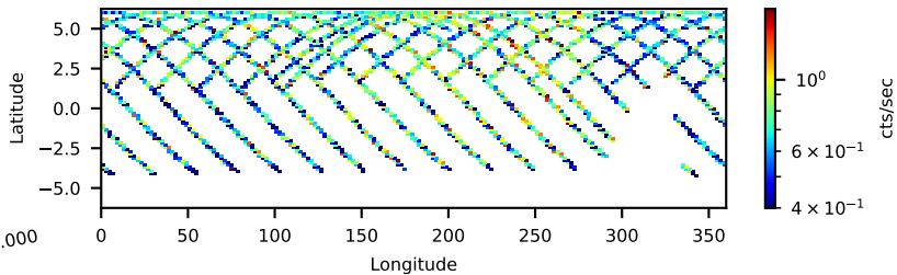
30302023004: 3 to 10 keV
