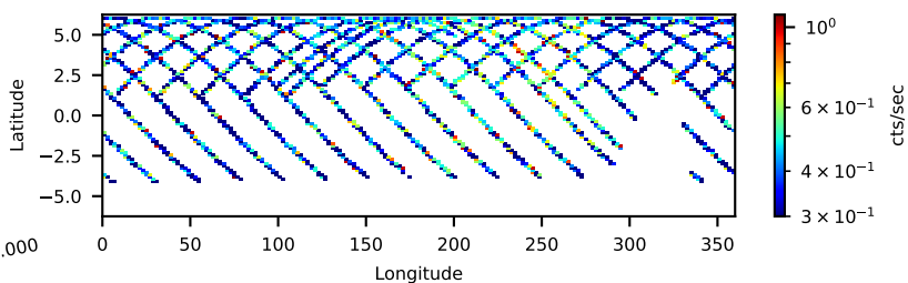
30302023004: 30 to 120 keV
