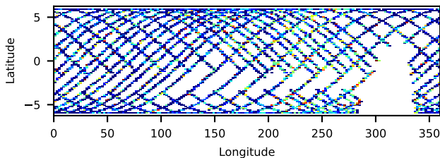
30302016002: 30 to 120 keV
