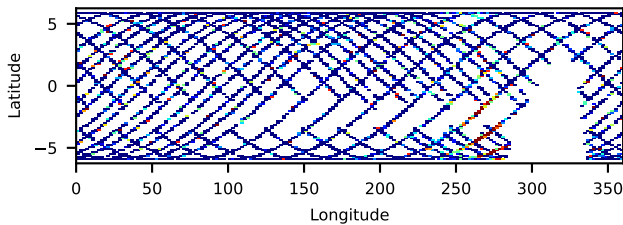
30302016002: 3 to 10 keV
