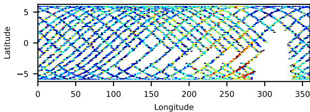
30302016002: 3 to 120 keV
