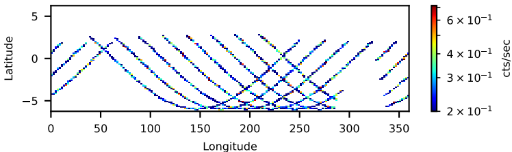
30101001002: 3 to 10 keV
