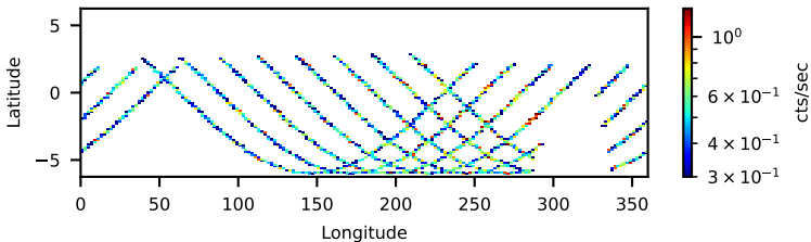
30101001002: 30 to 120 keV
