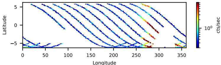
30002041020: 3 to 10 keV
