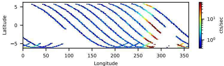
30002041020: 3 to 120 keV
