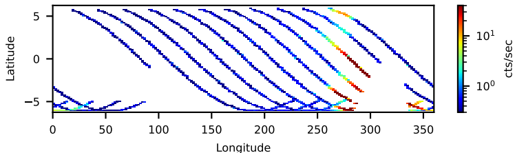
30002041020: 30 to 120 keV
