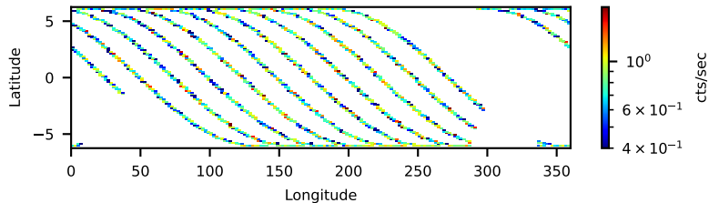
30002017002: 3 to 120 keV
