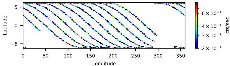
30002017002: 30 to 120 keV
