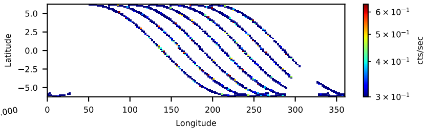
11001313002: 30 to 120 keV
