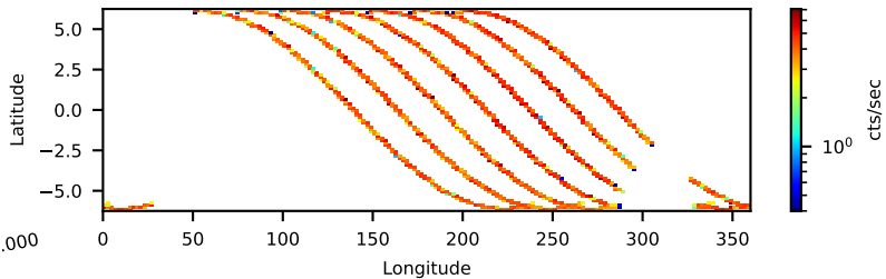
11001313002: 3 to 10 keV
