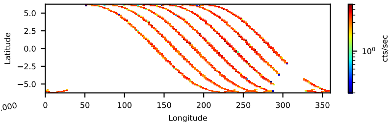
11001313002: 30 to 120 keV
