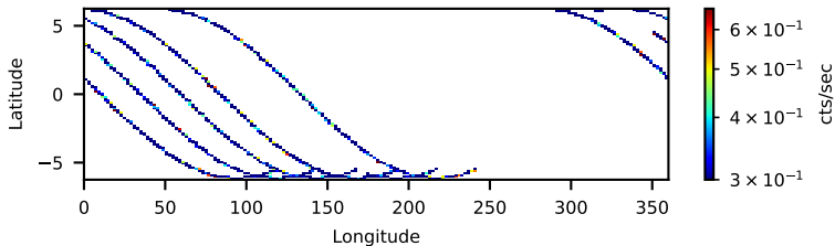
10902336002: 30 to 120 keV
