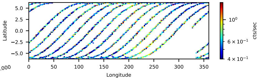
10802004002: 3 to 10 keV
