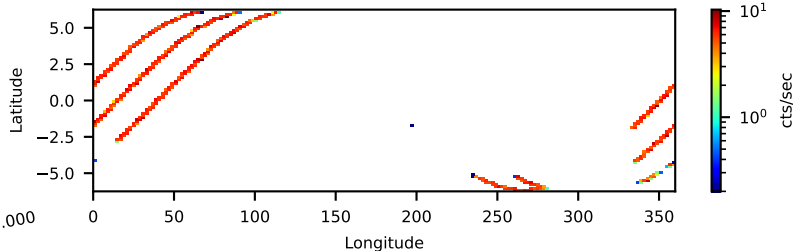
10602002008: 30 to 120 keV
