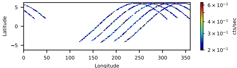
10502004004: 3 to 10 keV
