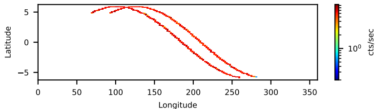
10502001002: 3 to 10 keV
