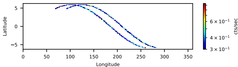
10502001002: 30 to 120 keV
