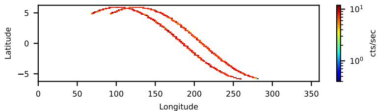
10502001002: 3 to 120 keV
