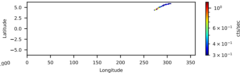
10013003001: 30 to 120 keV
