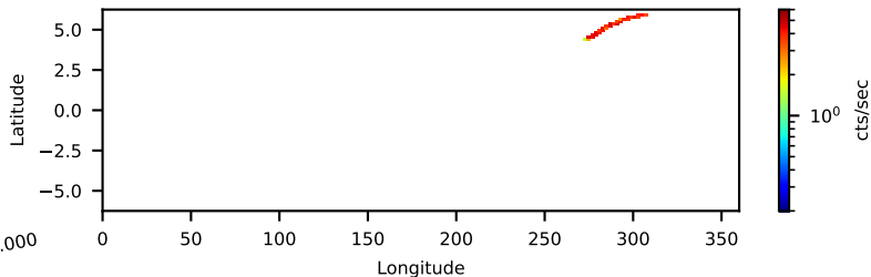
10013003001: 30 to 120 keV
