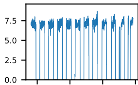
60-s bins
